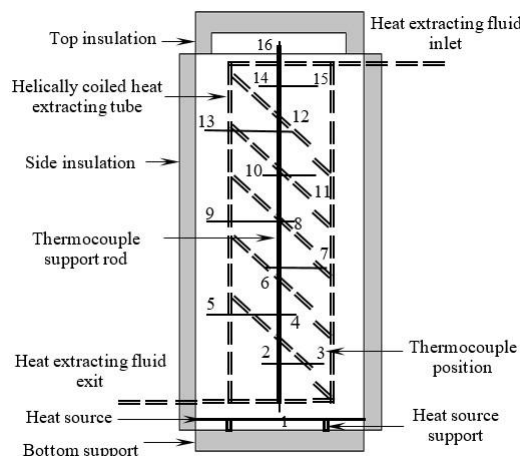
Figure 5: TES components and position of thermocouples.
