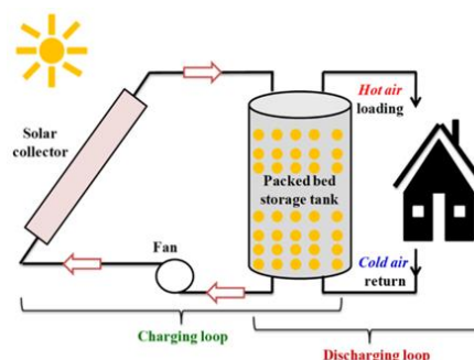
Figure 1: Packed bed TES with charging and discharging loops [8].
