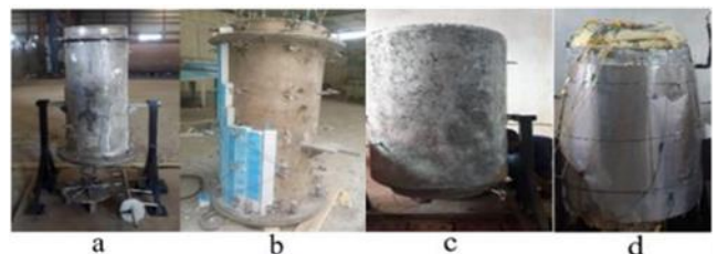
Figure 4: Thermal energy storage (TES) constructed with different insulation materials: a) TES without insulation, b) TES with refractory insulation, c) TES with Castable insulation over refractory, d) TES with fiberglass insulation over Castable insulation.
