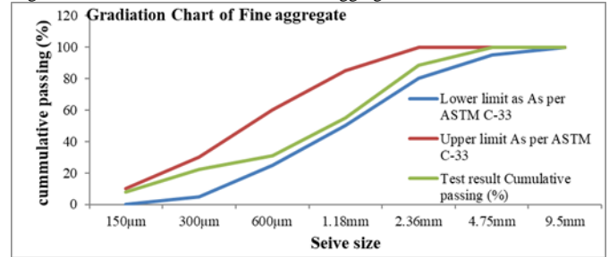
Figure 1. Particle size distribution of fine aggregates
